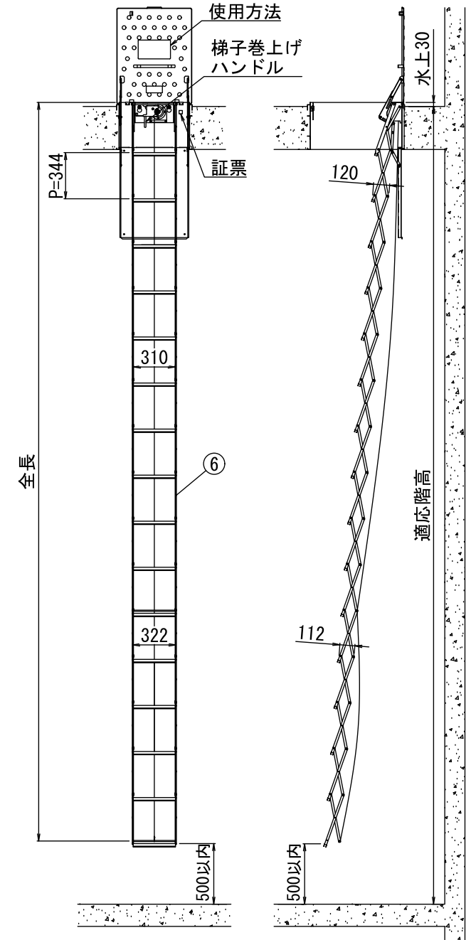
縮尺 (1:40)
